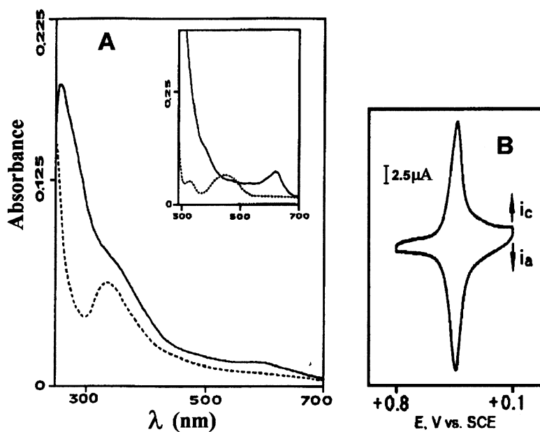
Fig. 7. (A) UV–vis spectra of a film of an ITO electrode modified with dendrimer 13 , measured after the film was oxidised at +0.70 V (—) and subsequently reduced at 0.0 V (---). Inset: UV–vis spectra of [\mathbf{13}^{8+}][\text{PF}_6^-] (—) and 13 (---) in \text{CH}_2\text{Cl}_2 solution, (B) cyclic voltammogram of an ITO electrode modified with a film of 13 measured in \text{CH}_2\text{Cl}_2/0.1 M TBAH (adapted from Refs. [19,43]).
