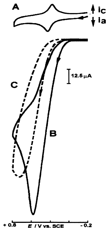
Fig. 4. Cyclic voltammogram in 0.1 M acetate buffer + 0.1 M \text{LiClO}_4 of: (A) a glassy carbon electrode modified with polymer 10 , (B) same electrode as in A with 10^{-3} M ascorbic acid, (C) a bare glassy carbon electrode in 10^{-3} M ascorbic acid (adapted from Ref. [45]).
