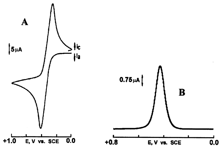
Fig. 5. (A) Cyclic voltammogram at a Pt disk electrode of dendrimer 13 in \text{CH}_2\text{Cl}_2/0.1 M TBAH solution, (B) differential pulse voltammogram of 13 in \text{CH}_2\text{Cl}_2/\text{CH}_3\text{CN} (14:1), 0.1 M TBAH solution.
